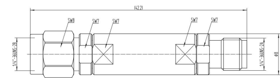
LT-LF-DC-27G-2.92MF
