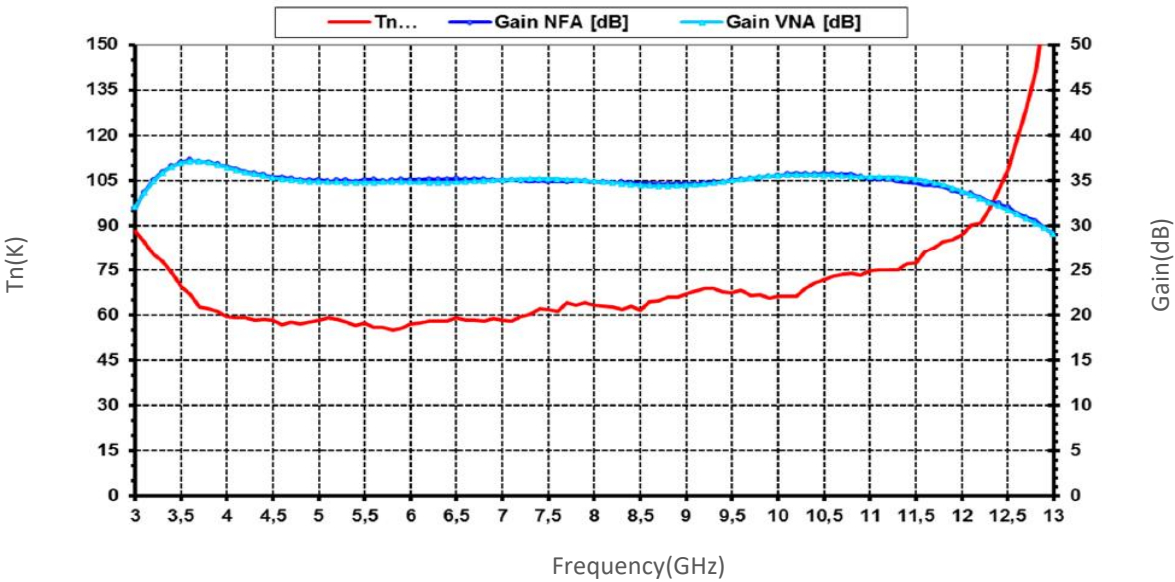
Noise Figure vs Frequency
