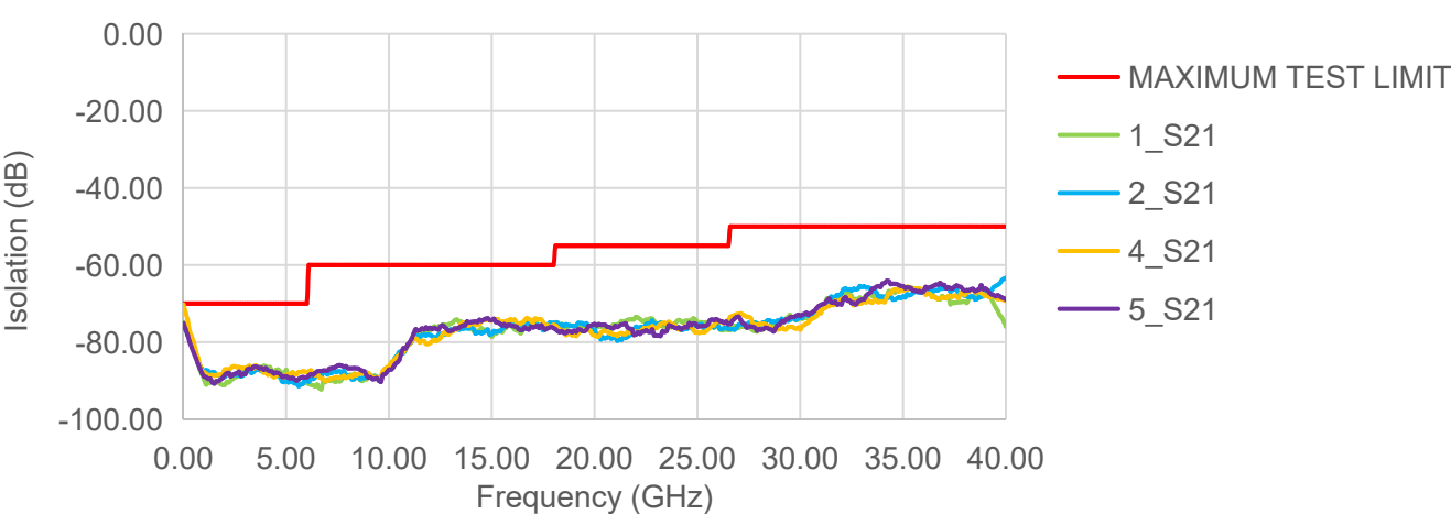
ISOLATION
