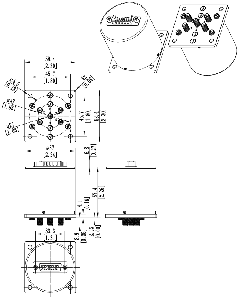
Outline Drawing: Unit: mm
