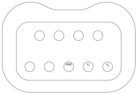
Nano D connector seen from outside the LNA
