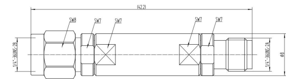
LT-LF-DC-1.5G-2.92MF
