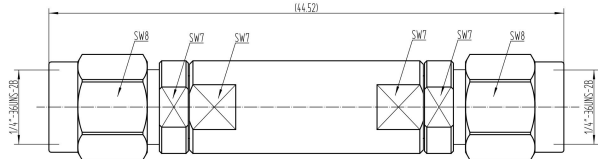
LT-LF-DC-1.5G-2.92MM
