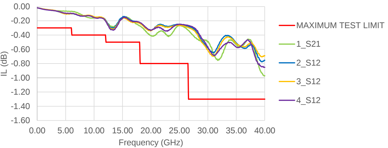
INSERTION LOSS
