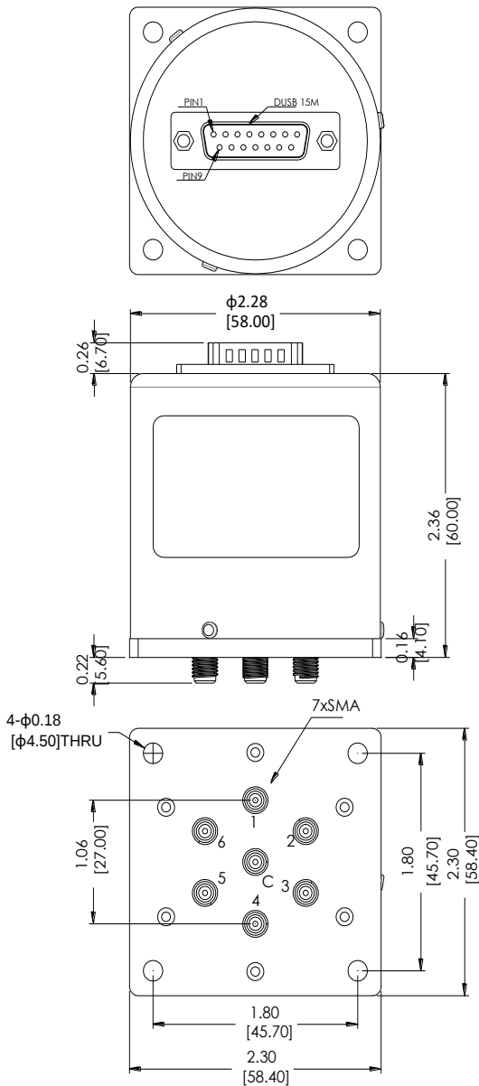
Outline Drawing:
