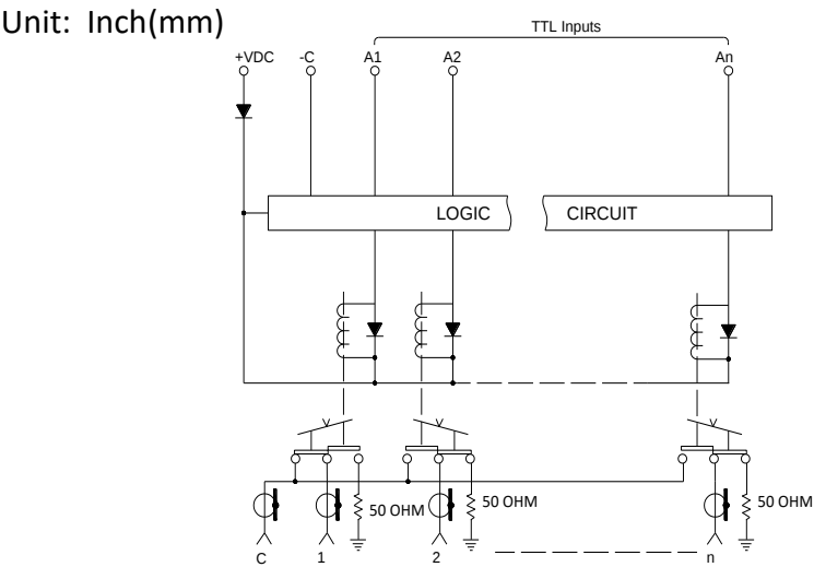
Schematic:
