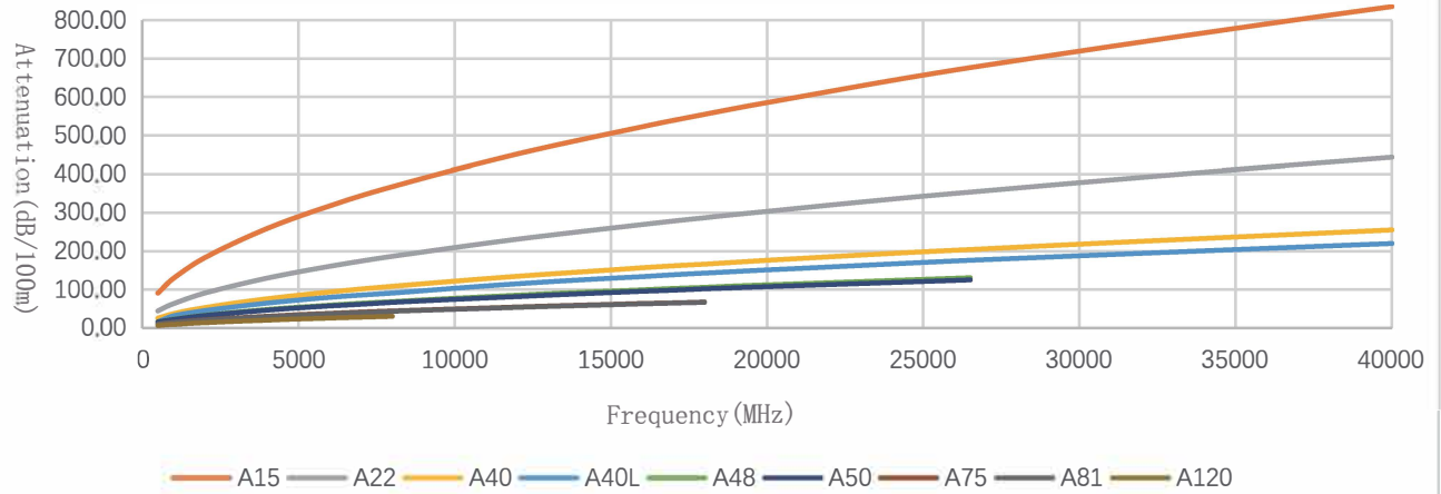
Attenuation VS Frequency
