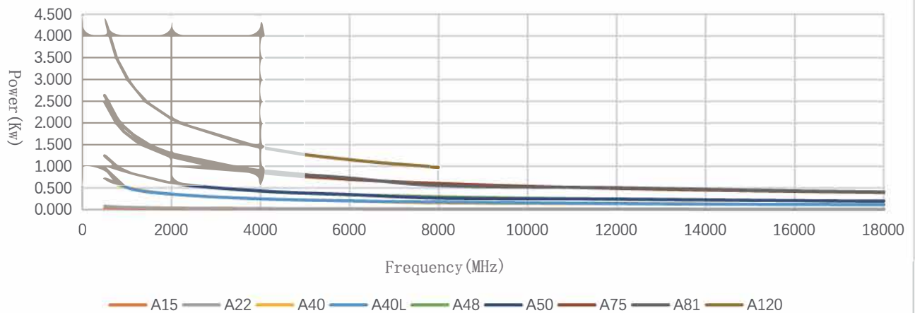
Power VS Frequency
