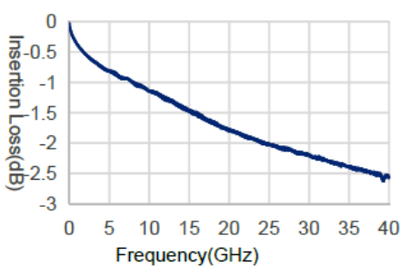
LT-A-C40-KMKM-1M Insertion Loss
