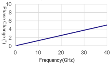
LT-A-C40 Phase VS Flexure
