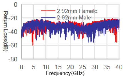
LT-A-C40-KMKM-1M Return Loss
