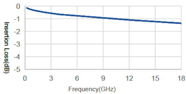
LT-A-C50-SMAMKM-XM Insertion Loss
