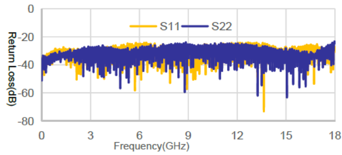
LT-A-C50-SMAMKM-XM Return Loss
