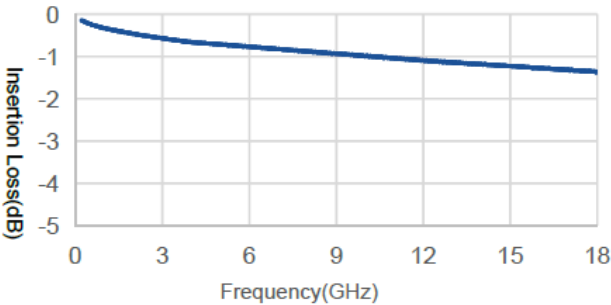
LT-A-C50-SMAMSMAM-XM Insertion Loss
