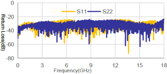
LT-A-C50-SMAMSMAM-XM Return Loss
