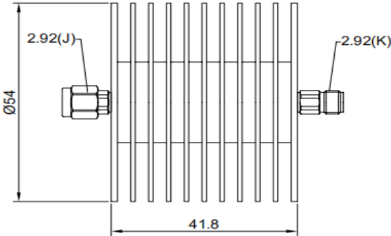
40db Outline dimensions
