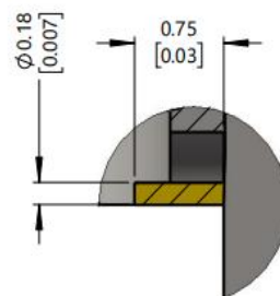
DETAIL A(20:1)
